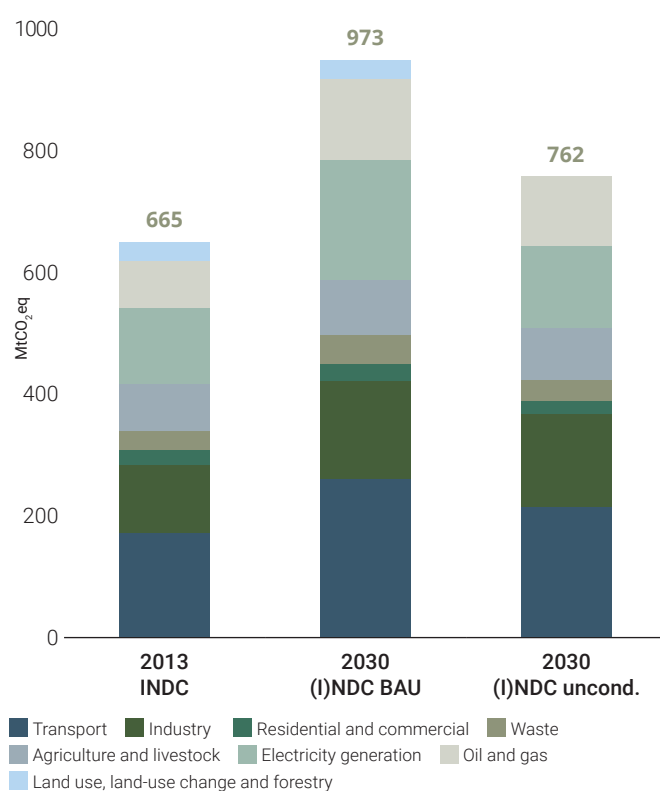
MEXICO’S NDC MITIGATION TARGETS BY SECTOR (ECKSTEIN ET AL. 2020) (FIGURE 6)
